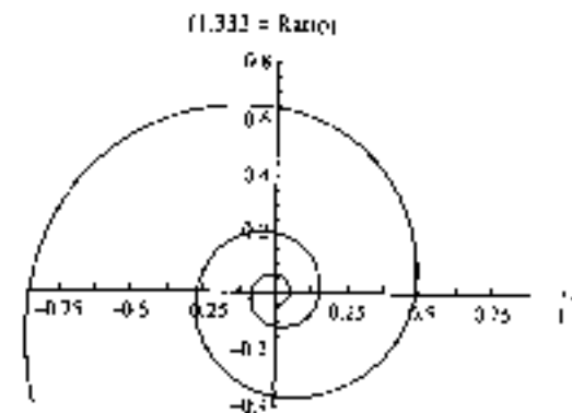
Figure 3. A spiral with a 1.33 to 1 ratio
